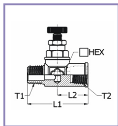
流量調節閥 Flow Control Valve
